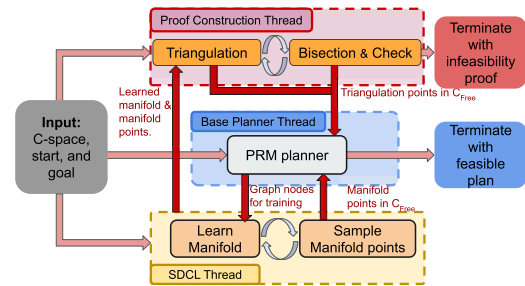
Fig. 1. Algorithm overview. Three threads run in parallel. The algorithm terminates with a plan or an infeasibility proof.
